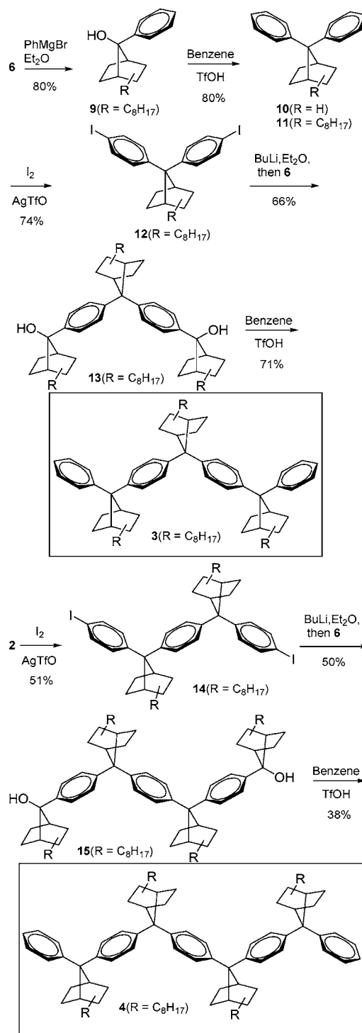
Scheme 2. Synthesis of DFN Trimer 3 and Tetramer 4
