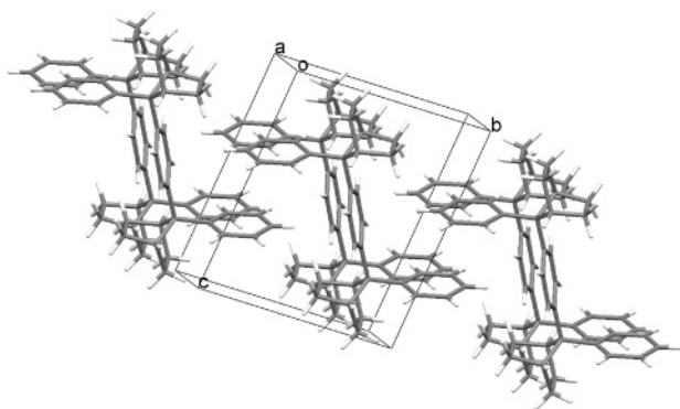
Figure 2. Crystal packing of dimer 1 .
