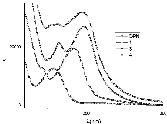
Figure 3. Electronic spectra in hexane of DPN, 1 , 3 , and 4 .
