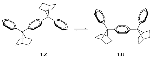
Figure 1. Z- and U-shaped conformers of dimer 1 .
