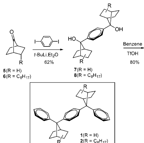
Scheme 1. Synthesis of DFN Dimers 1 and 2
